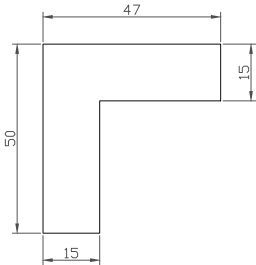
Standard Corner Fitting - Face Mounted Scale 1:1
