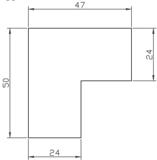
Standard Corner Fitting - Flush Fitting Scale 1:1
